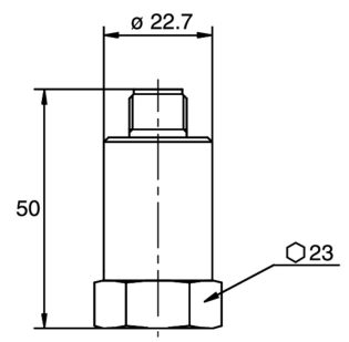
Housing with connector M12-A, 4-pin
