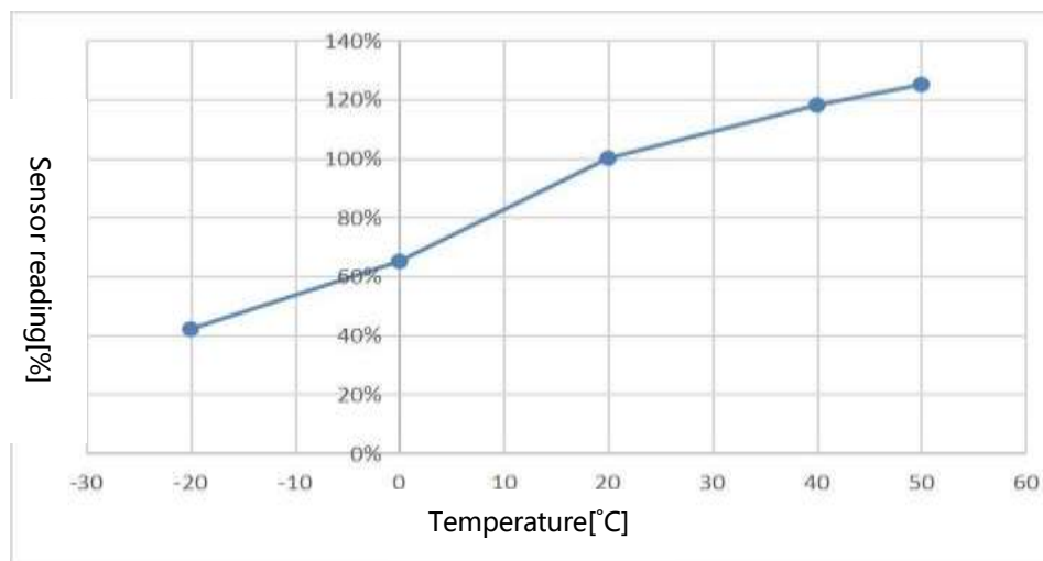
Figure 2: Temperature supplement compensation curve
