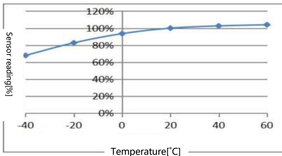
Figure 2: Temperature supplement compensation curve
