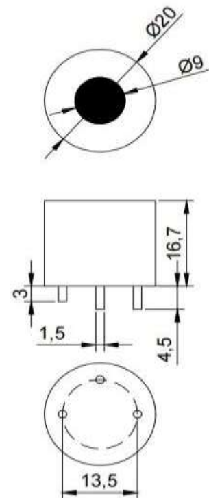
Figure 1: Unit: mm Unless otherwise specified, all tolerances are ±0.1mm.
