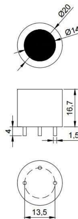
Figure 1: Unit: mm Unless otherwise specified, all tolerances are \pm 0.1 mm.
