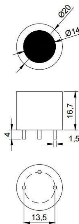
Figure 1: Unit: mm Unless otherwise specified, all tolerances are ±0.1mm.
